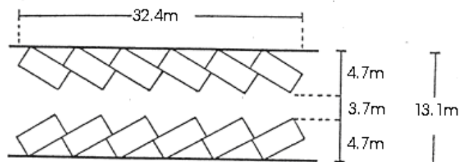
30° PARKING
