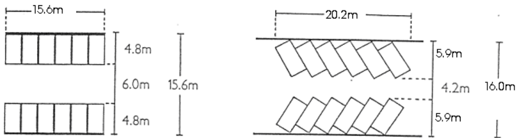
90° PARKING
