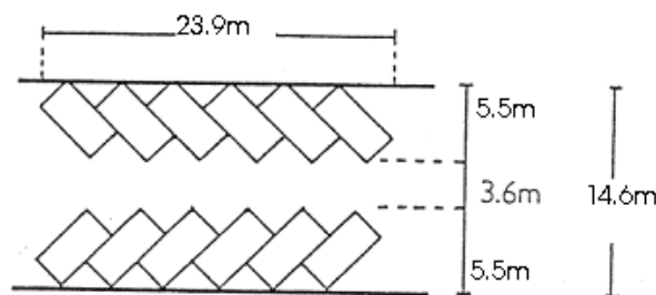
45° PARKING
